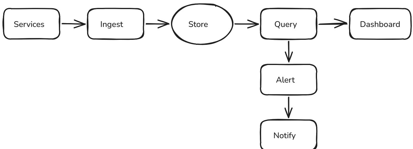
Data Flow
